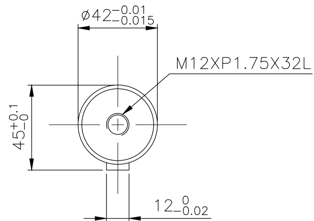
A VIEW
